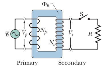
Figure 31-18 An ideal transformer (two coils wound on an iron core) in a basic transformer circuit. An ac generator produces current in the coil at the left (the primary ). The coil at the right (the secondary ) is connected to the resistive load R when switch S is closed.
