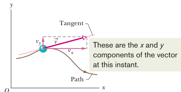
Figure 4-4 The velocity \vec{v} of a particle, along with the scalar components of \vec{v} .
