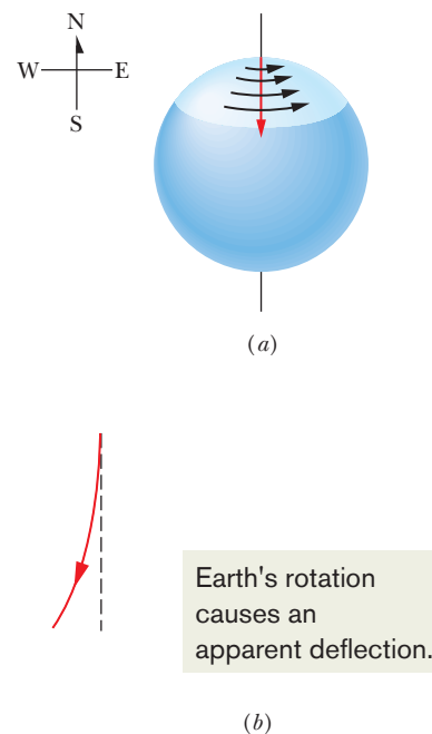
Figure 5-2 (a) The path of a puck sliding from the north pole as seen from a stationary point in space. Earth rotates to the east. (b) The path of the puck as seen from the ground.
