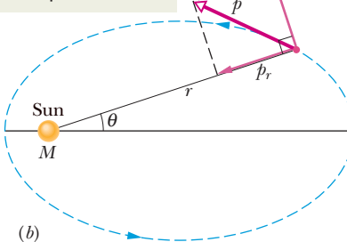
Figure 13-13 (a) In time \Delta t , the line r connecting the planet to the Sun moves through an angle \Delta\theta , sweeping out an area \Delta A (shaded). (b) The linear momentum \vec{p} of the planet and the components of \vec{p} .
