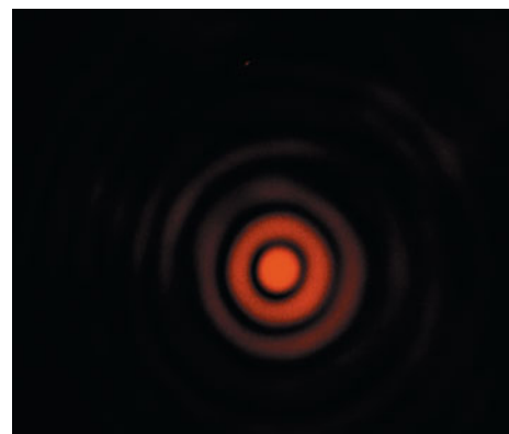
Figure 36-3 A photograph of the diffraction pattern of a disk. Note the concentric diffraction rings and the Fresnel bright spot at the center of the pattern. This experiment is essentially identical to that arranged by the committee testing Fresnel's theories, because both the sphere they used and the disk used here have a cross section with a circular edge.
