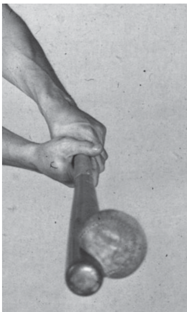
The collision of a ball with a bat collapses part of the ball.
