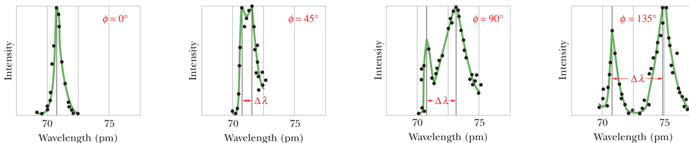
Figure 38-4 Compton's results for four values of the scattering angle \phi . Note that the Compton shift \Delta\lambda increases as the scattering angle increases.
