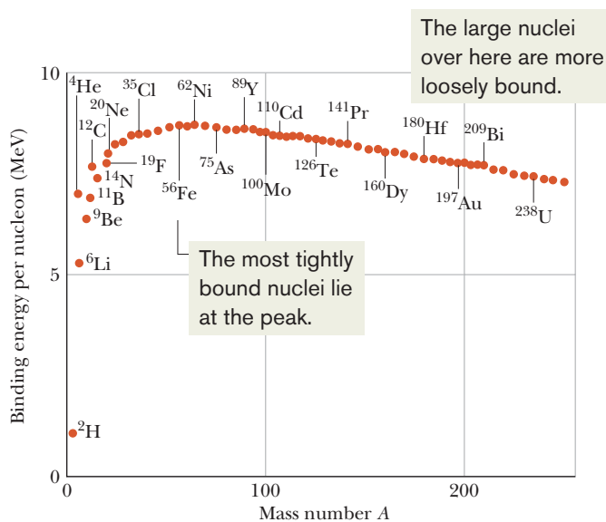
Figure 42-7 The binding energy per nucleon for some representative nuclides. The nickel nuclide {}^{62}\text{Ni} has the highest binding energy per nucleon (about 8.794 60 MeV/nucleon) of any known stable nuclide. Note that the alpha particle ( {}^4\text{He} ) has a higher binding energy per nucleon than its neighbors in the periodic table and thus is also particularly stable.
