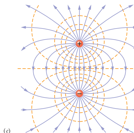
Figure 24-5 Electric field lines (purple) and cross sections of equipotential surfaces (gold) for (a) a uniform electric field, (b) the field due to a charged particle, and (c) the field due to an electric dipole.
