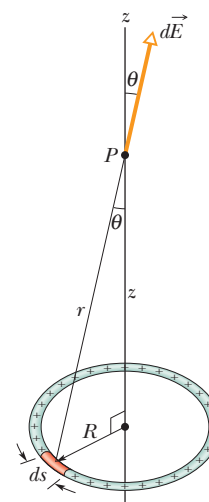
Figure 22-11 A ring of uniform positive charge. A differential element of charge occupies a length ds (greatly exaggerated for clarity). This element sets up an electric field d\vec{E} at point P .
