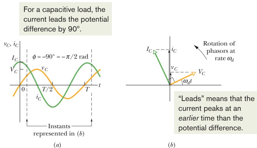
Figure 31-11 (a) The current in the capacitor leads the voltage by 90^\circ (= \pi/2 \text{ rad}) . (b) A phasor diagram shows the same thing.
