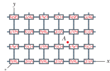
Figure 37-3 One section of a three-dimensional array of clocks and measuring rods by which an observer can assign spacetime coordinates to an event, such as a flash of light at point A . The event’s space coordinates are approximately x = 3.6 rod lengths, y = 1.3 rod lengths, and z = 0 . The time coordinate is whatever time appears on the clock closest to A at the instant of the flash.
