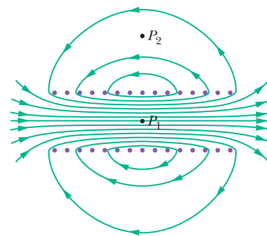
Figure 29-19 Magnetic field lines for a real solenoid of finite length. The field is strong and uniform at interior points such as P_1 but relatively weak at external points such as P_2 .
